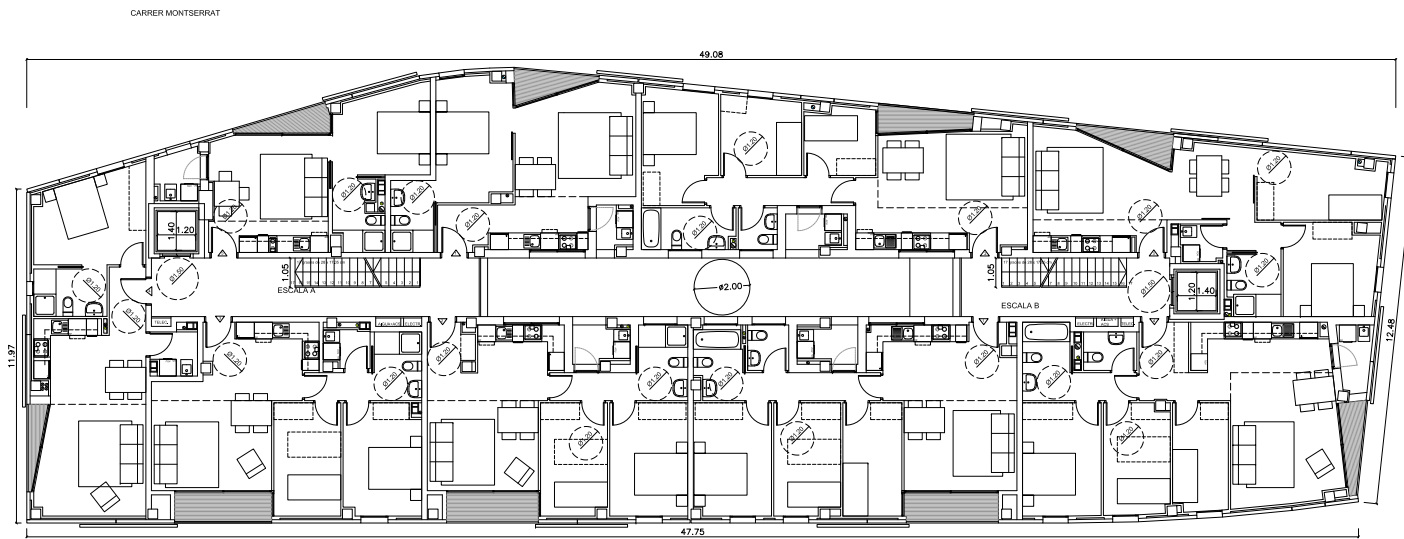
PLANTA QUARTA +232.90
