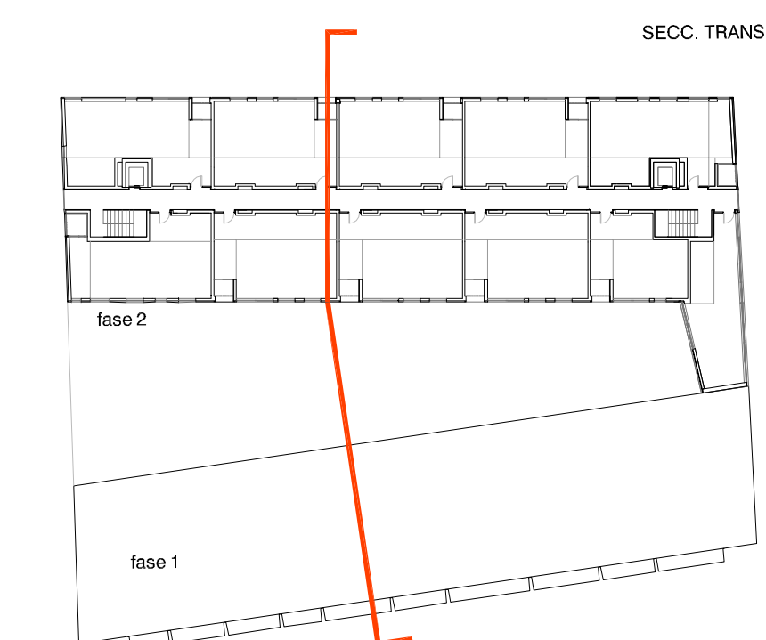
SECC. TRANS. 2
